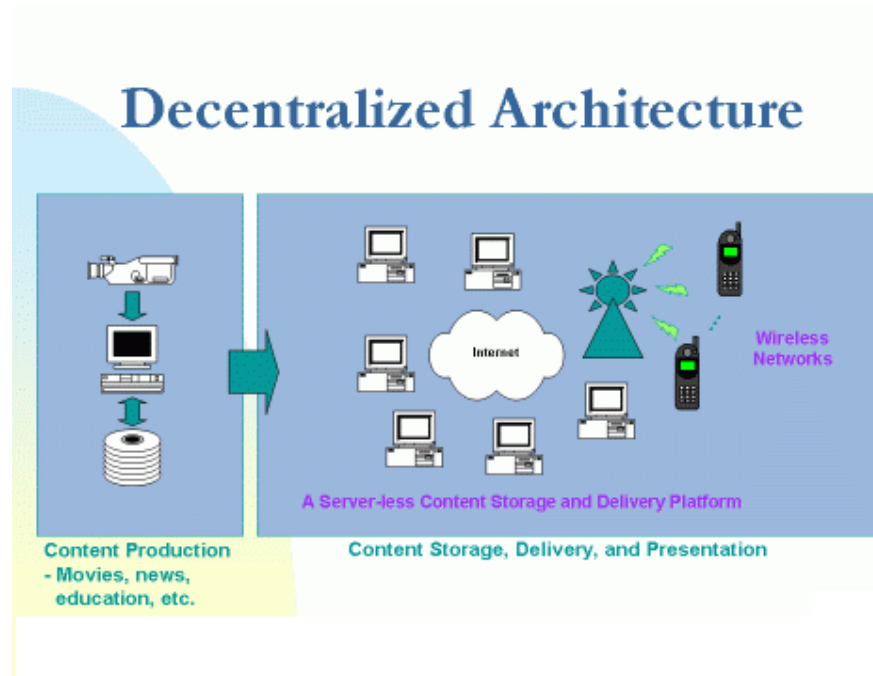
Figure.2: Decentralized architecture
